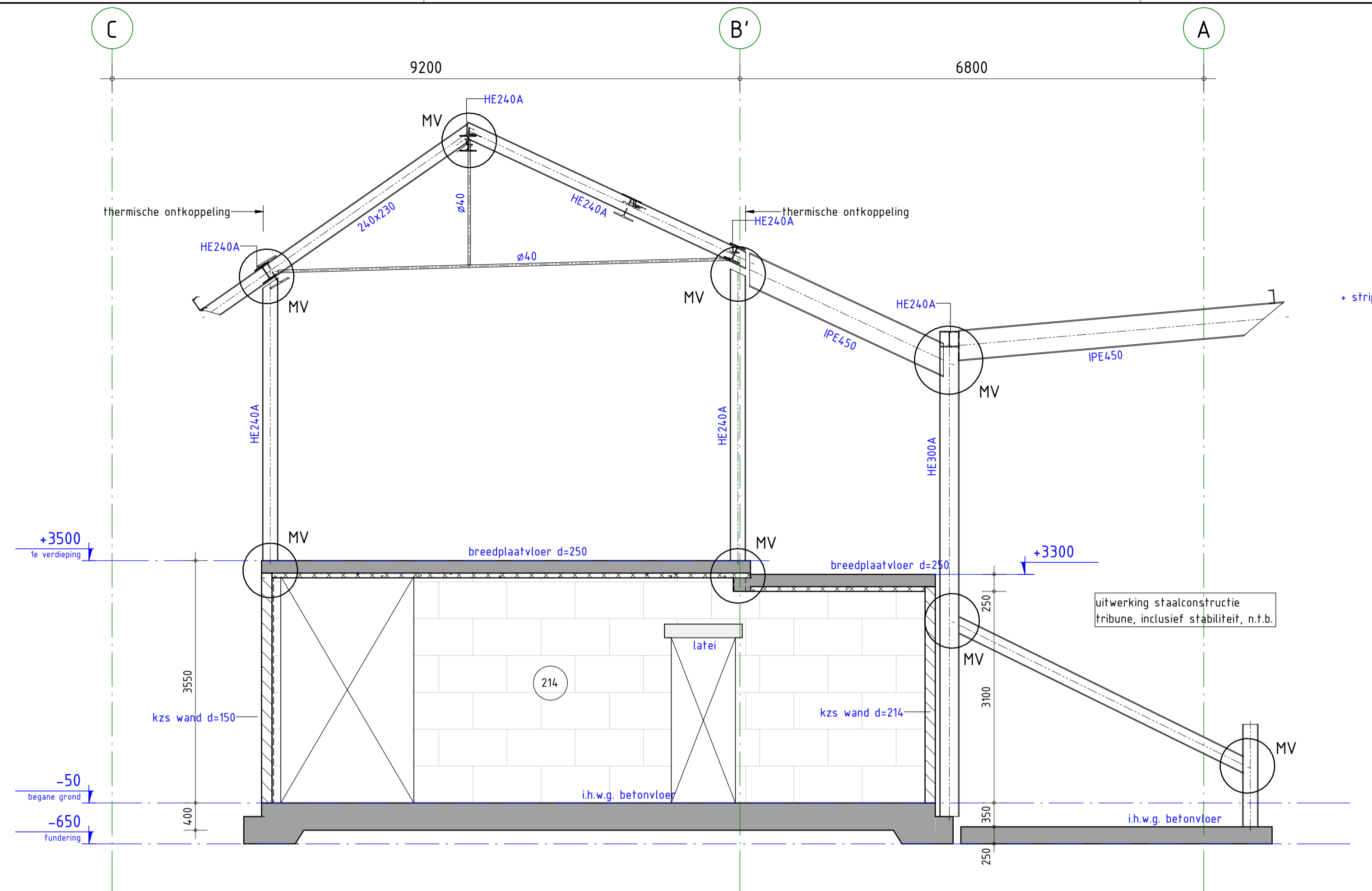
Doorsnede as 2
