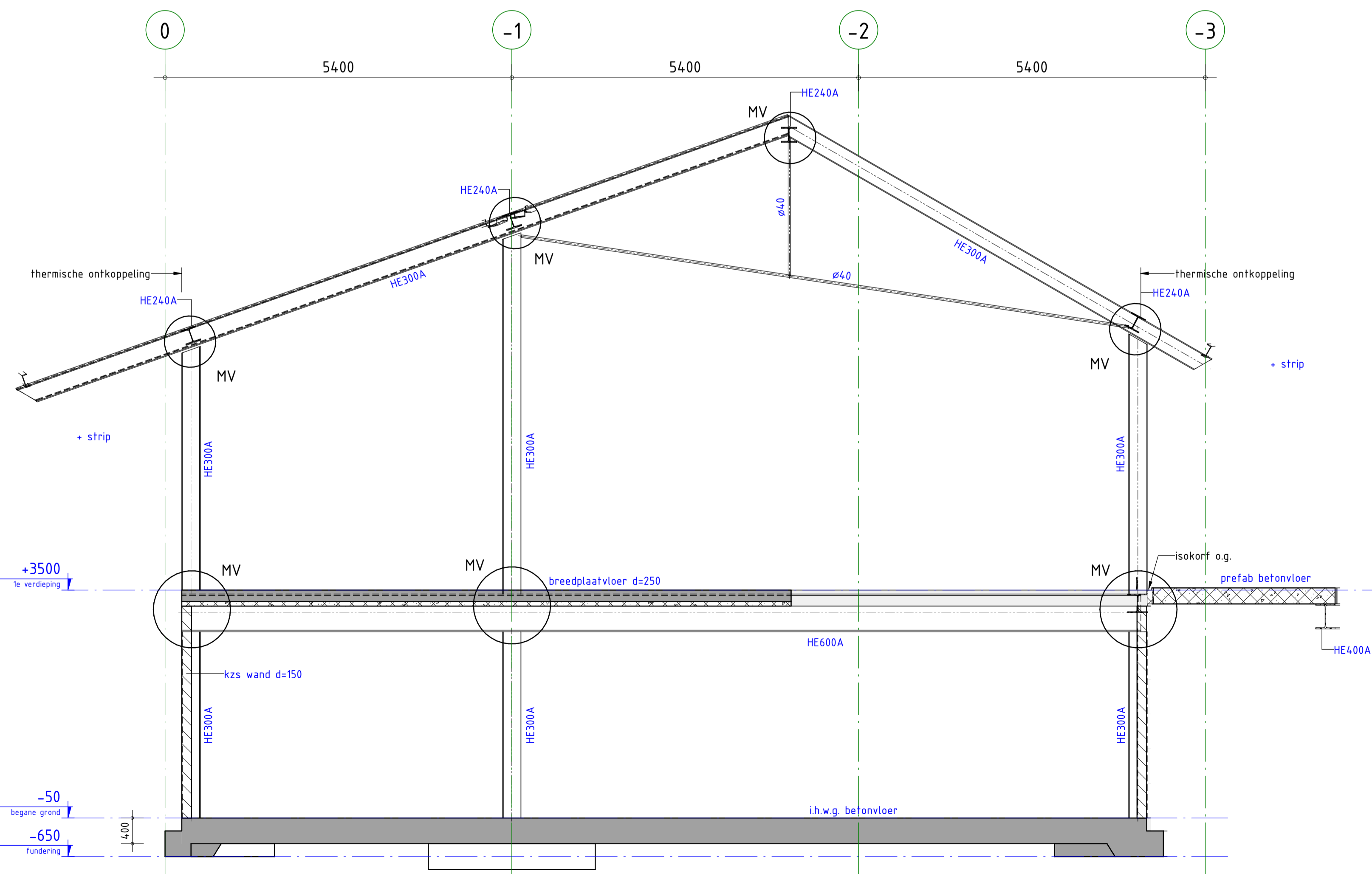
Doorsnede as F
