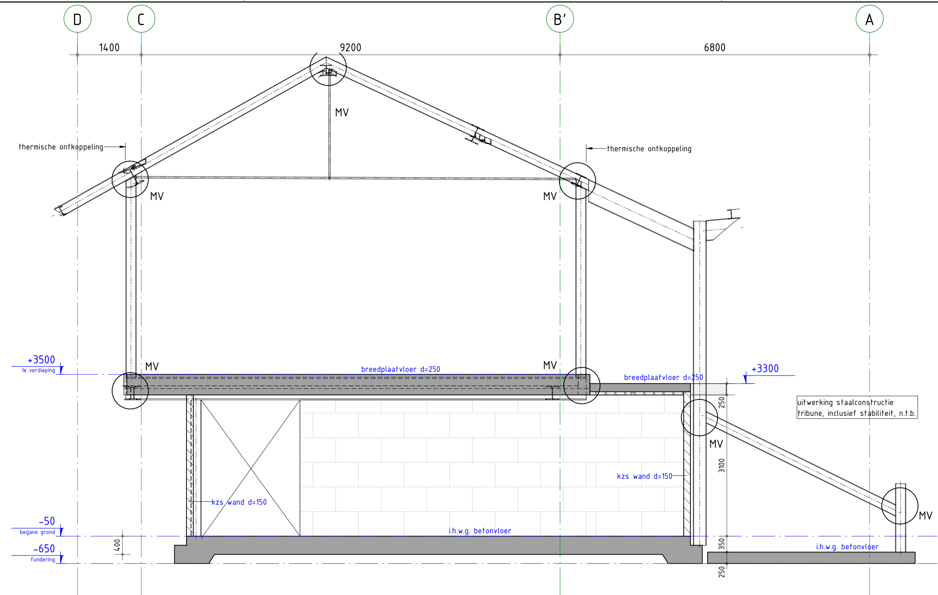
Doorsnede as -5
